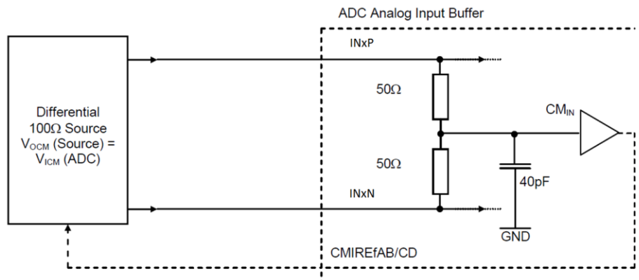
Figure 21: Differential analog input implementation (DC coupled)
