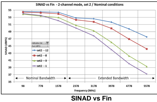
Figure 64: Performance vs Analog input frequencies - 2-channel mode – 3.2 GSps - Calibration set: CalSet2 -
