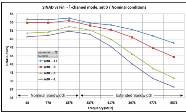
Figure 65: Performance vs Analog input frequencies - 1-channel mode – 6.4 GSps - Calibration set: CalSet0 -
