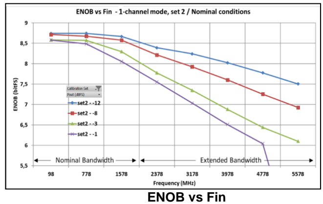
Figure 66: Performance vs Analog input frequencies - 1-channel mode – 6.4 GSps - Calibration set: CalSet2 -
