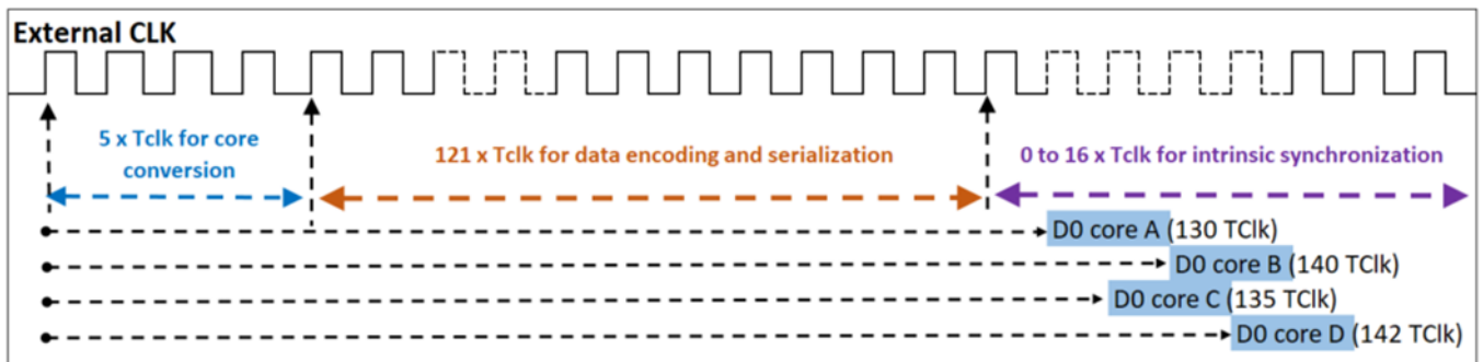
Figure 6: Latency example 2
