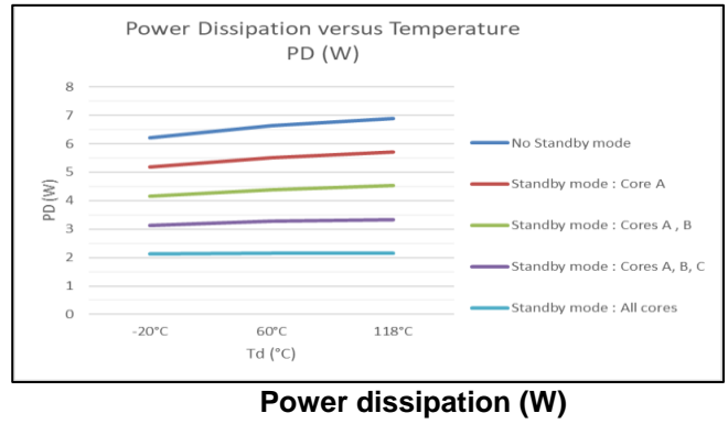
Figure 48: Current consumption and power dissipation versus temperature and standby mode
