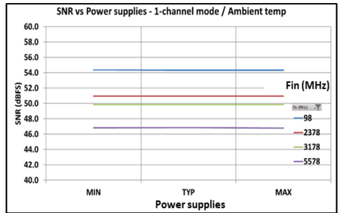
SNR vs power supplies
