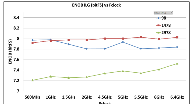
ENOB vs Fclock
