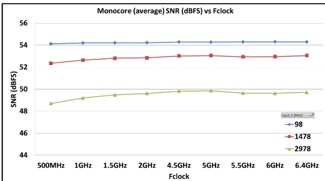
SNR vs Fclock
