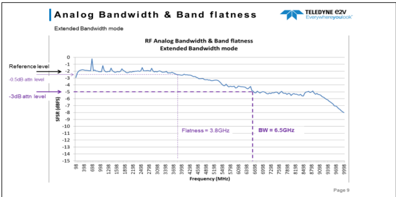
Figure 50: Extended Bandwidth
