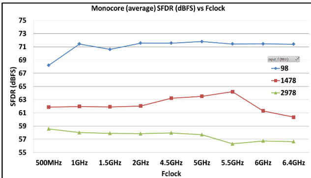
SFDR vs Fclock
