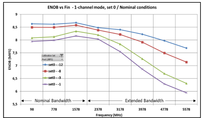
Figure 65: Performance vs Analog input frequencies - 1-channel mode – 6.4 GSps - Calibration set: CalSet0 -
