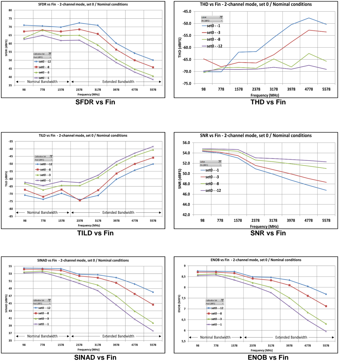
Figure 63: Performance vs Analog input frequencies - 2-channel mode – 3.2 GSps - Calibration set: CalSet0 -
