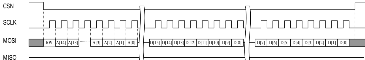
Figure 13: SPI writing
