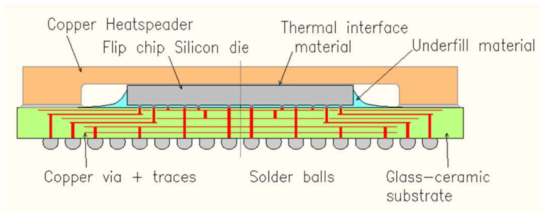
Figure 7: Package cross-section
