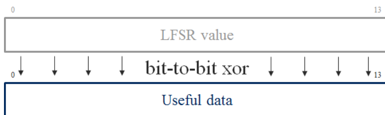
Figure 38: LFSR operation
