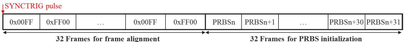
Figure 36: Synchronization sequence
