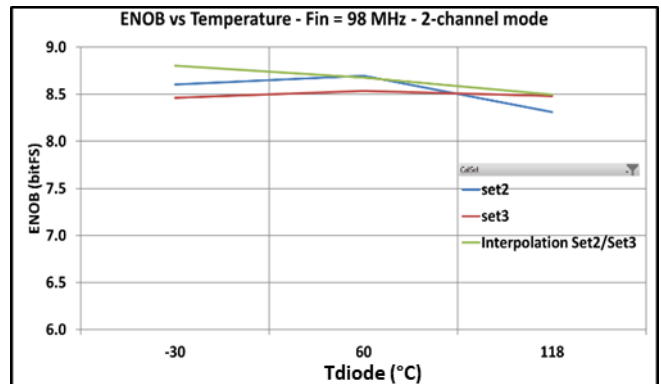
ENOB vs temperature
