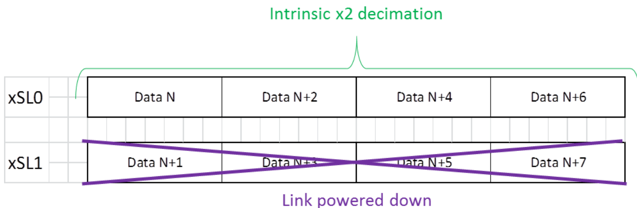
Figure 27: Powering down 1 link gives a x2 decimation.
