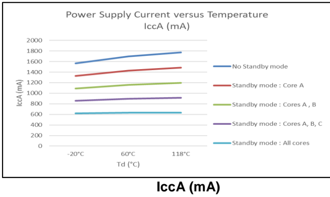
Figure 48: Current consumption and power dissipation versus temperature and standby mode
