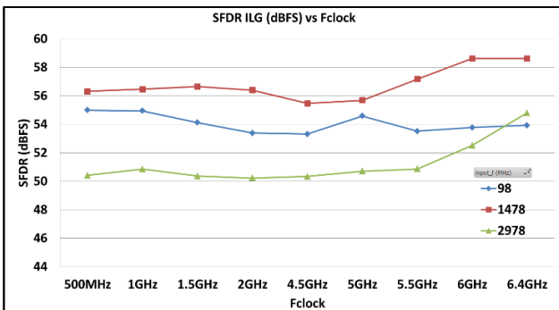
SFDR vs Fclock
