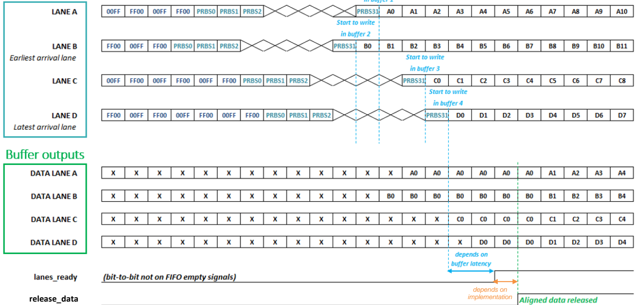
Figure 41: Multi-lanes synchronization time chart principle
