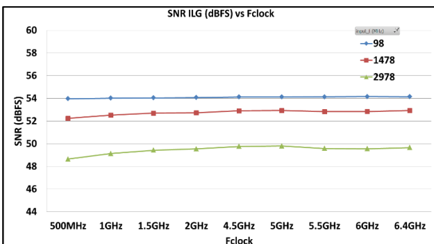
SNR vs Fclock
