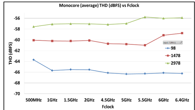
THD vs Fclock
