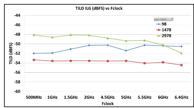
TILD vs Fclock
