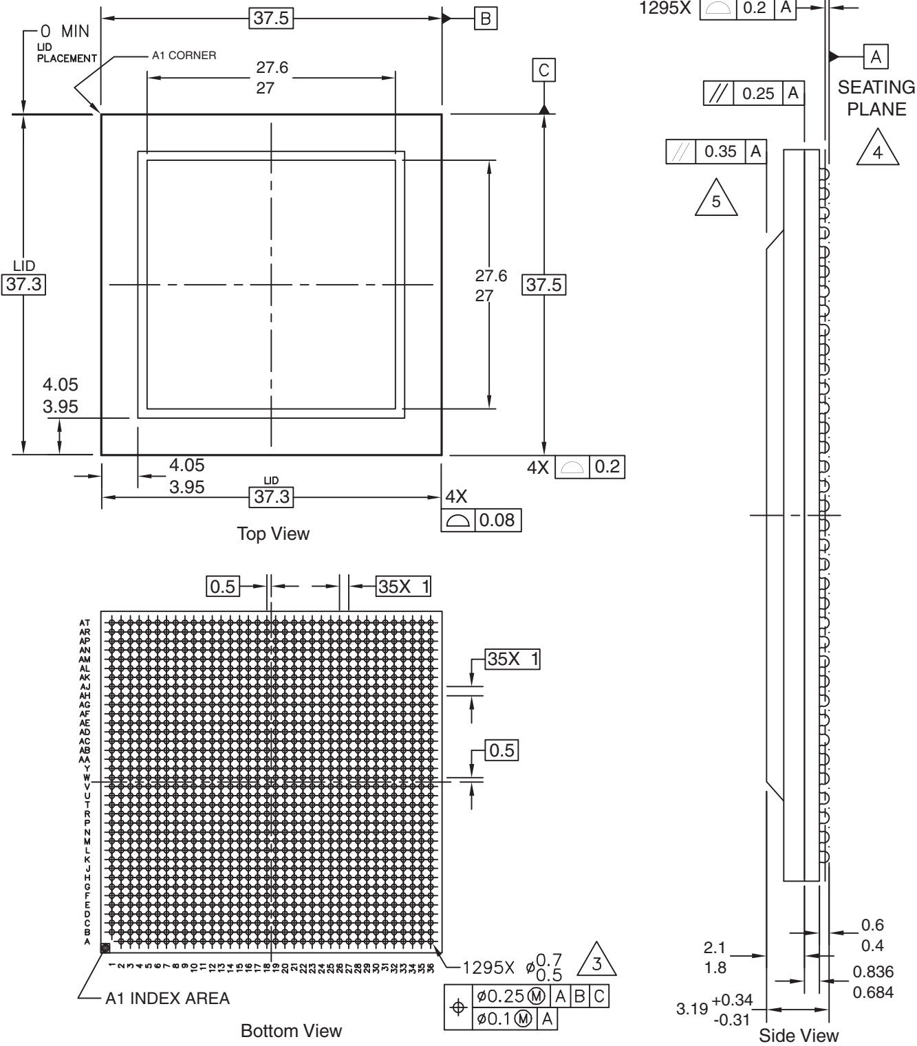
Figure 4-1. Mechanical Dimensions of the P4040 FC-PBGA with Full Lid
