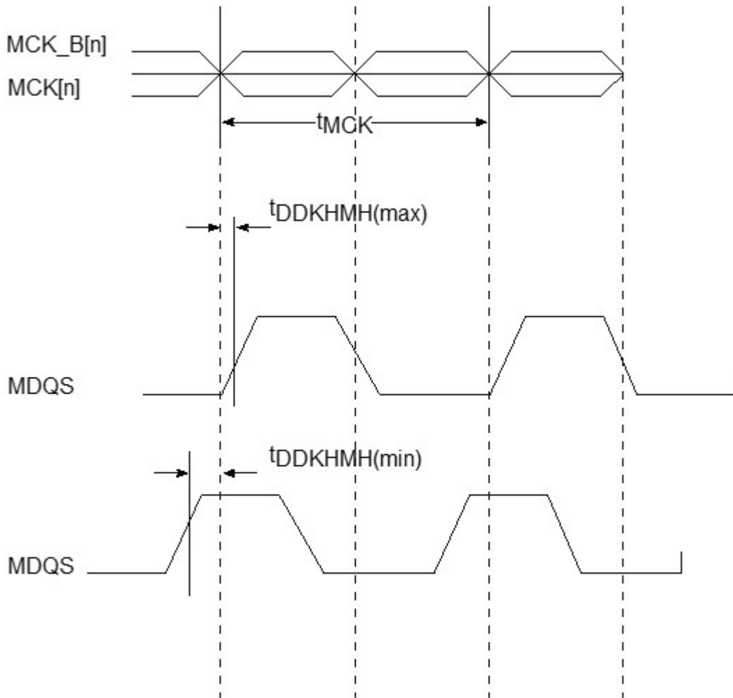
Figure 13. t_{DDKHMH} timing diagram
