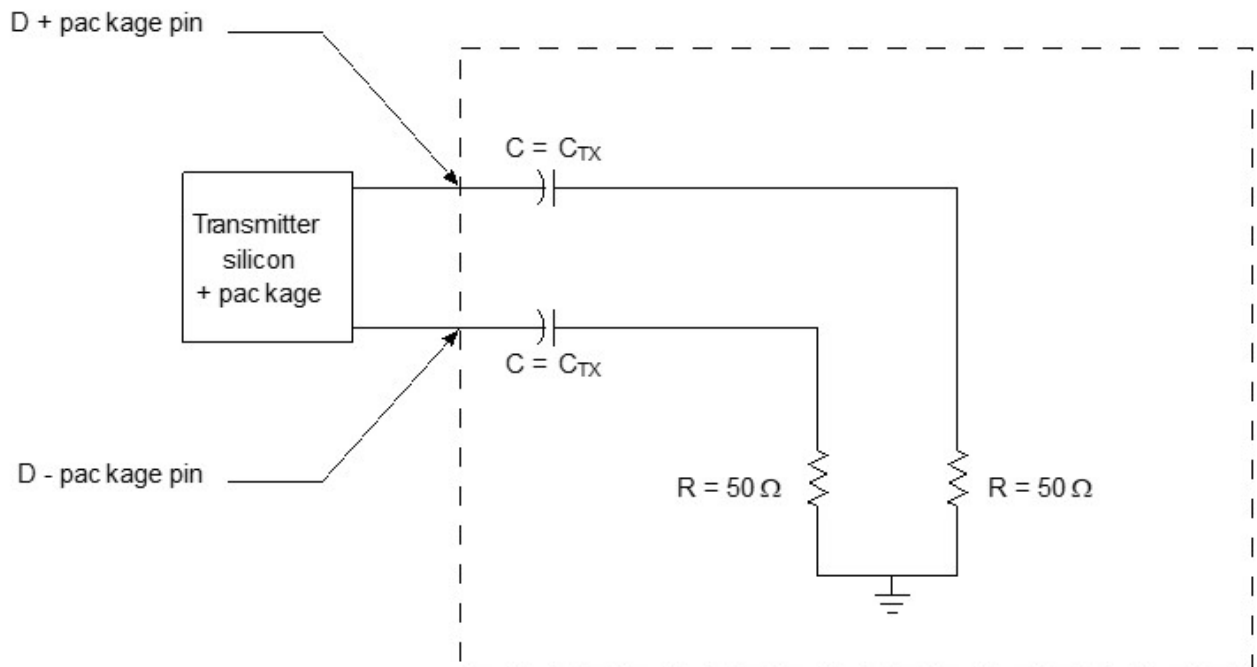
Figure 17. SGMII AC test/measurement load
