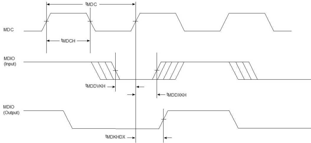
Figure 22. Ethernet management interface 1 timing diagram
