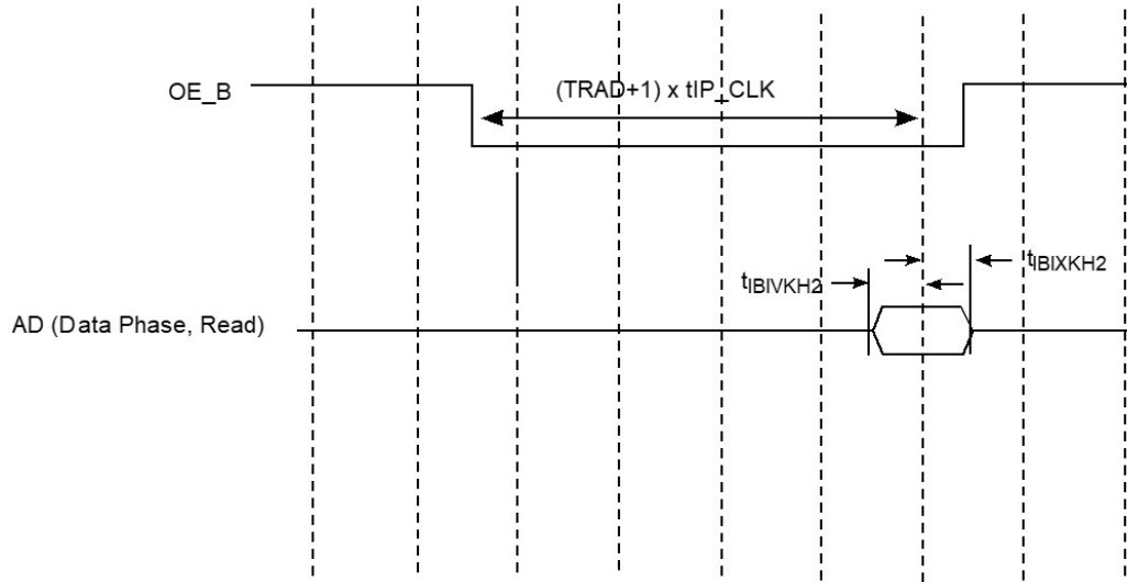
Figure 30. IFC-NOR interface input AC timings
