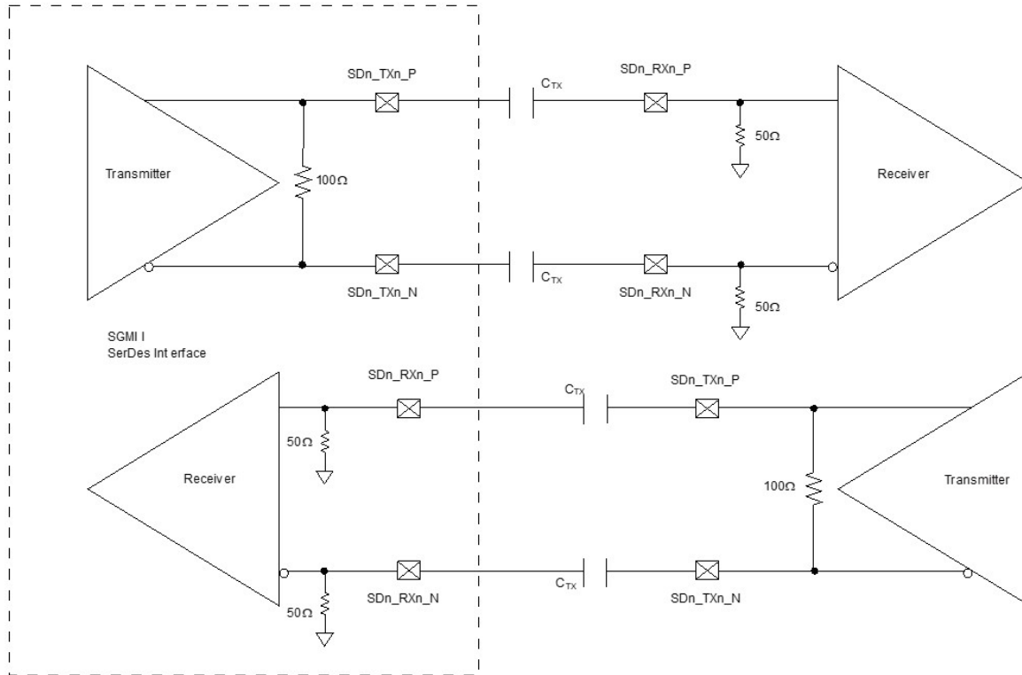
Figure 15. 4-wire AC-coupled SGMII serial link connection example
