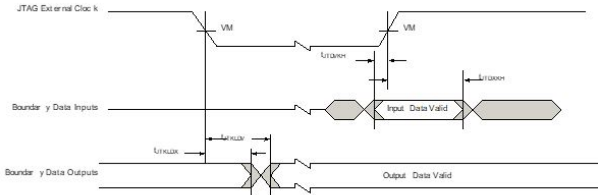
Figure 74. Boundary-scan timing diagram
