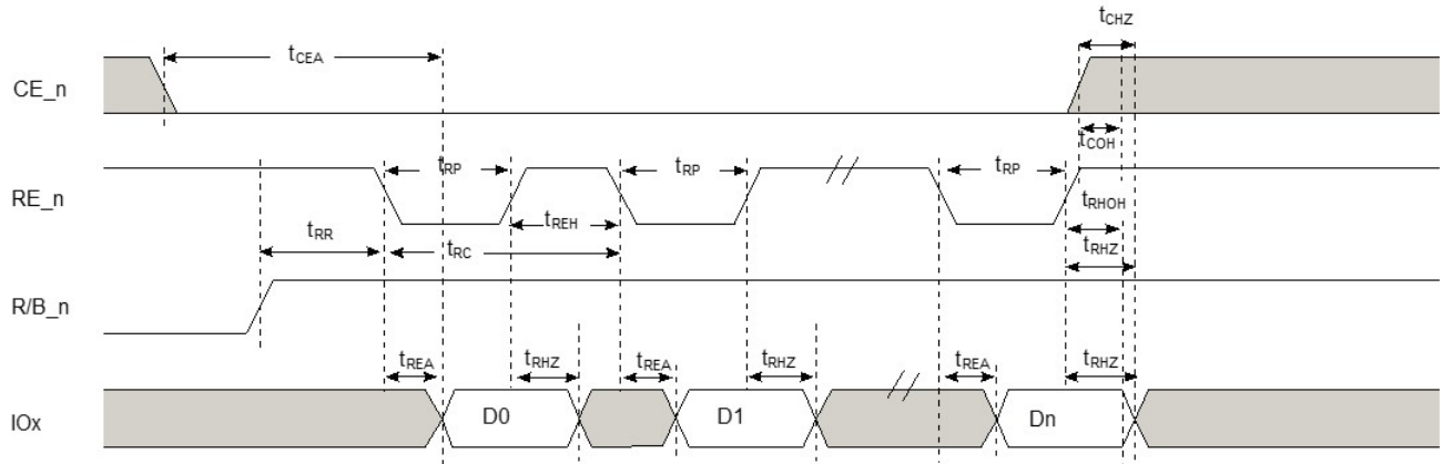
Figure 37. Data input cycle timings
