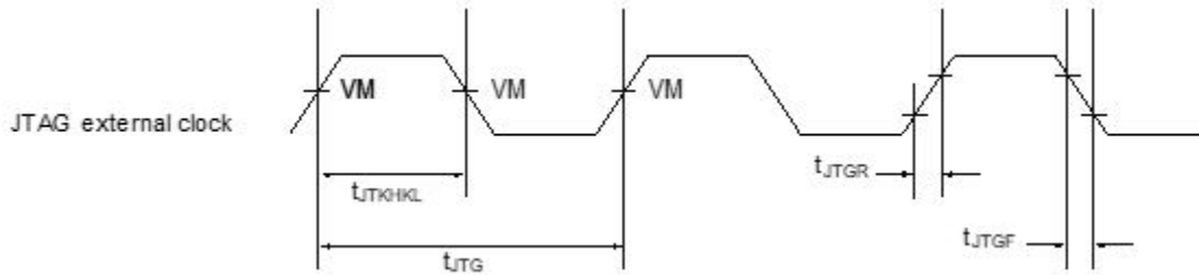
Figure 72. JTAG clock input timing diagram
