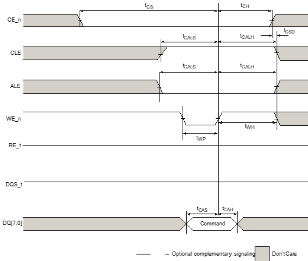
Figure 35. Command cycle
