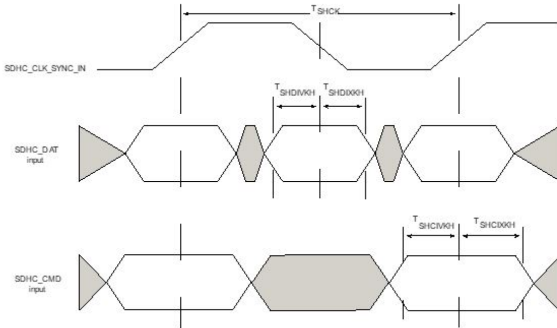
Figure 68. eSDHC DDR50/DDR mode input AC timing diagram
