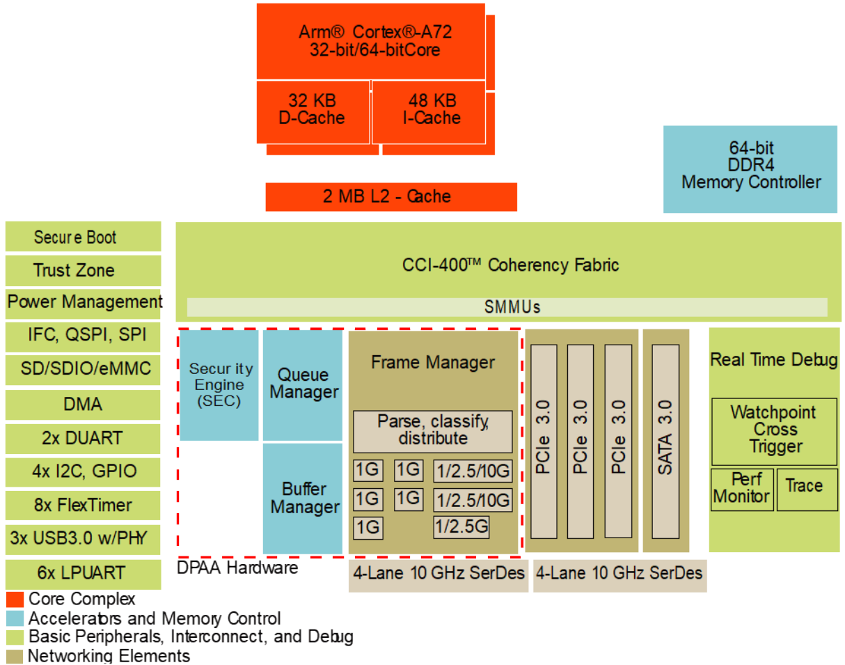
Figure 2. LS1026A block diagram
