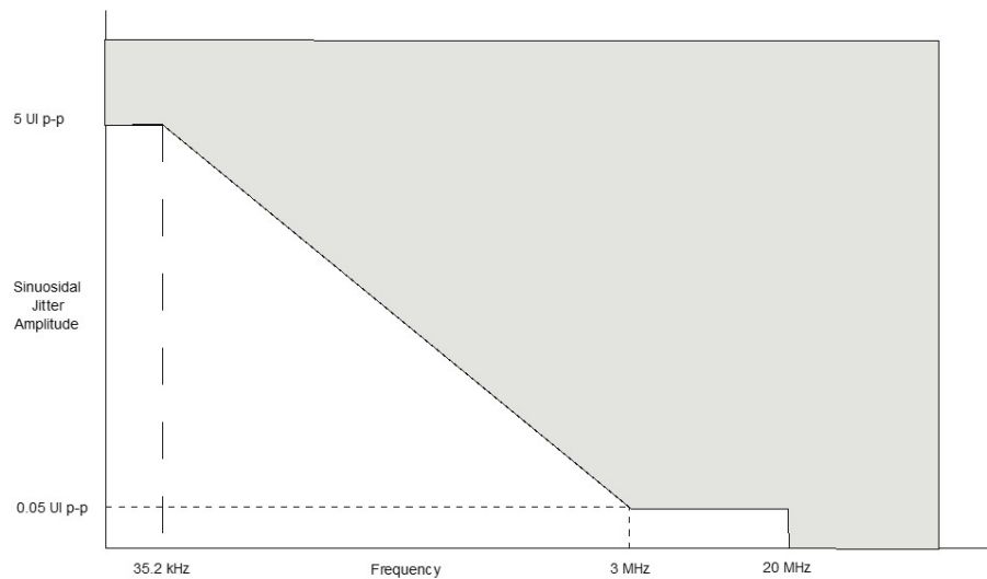
Figure 19. QSGMII single-frequency sinusoidal jitter limits
