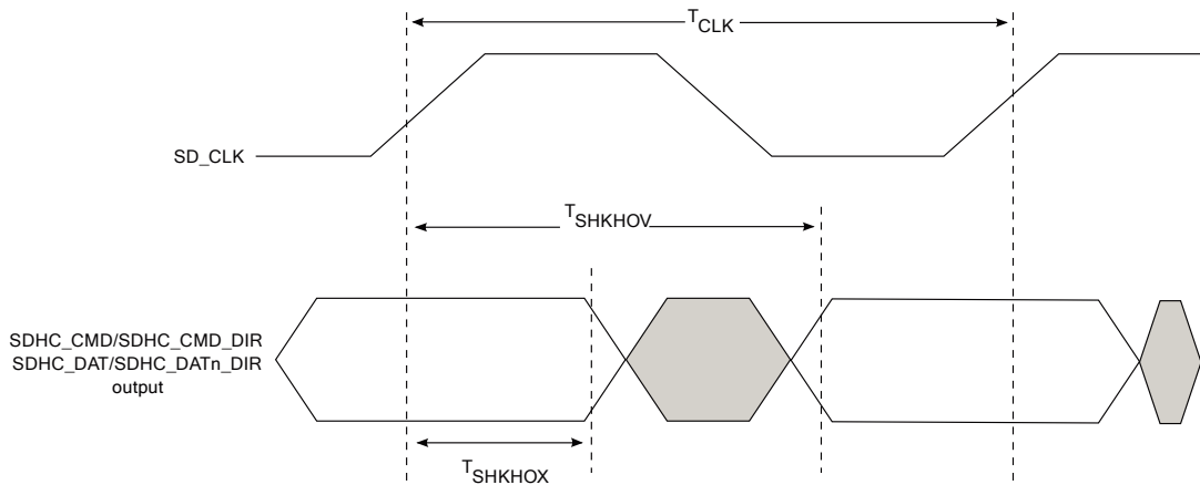
Figure 67. eSDHC SDR50 mode output timing diagram
