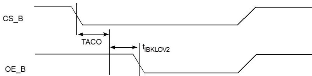
Figure 31. IFC-NOR interface output AC timings
