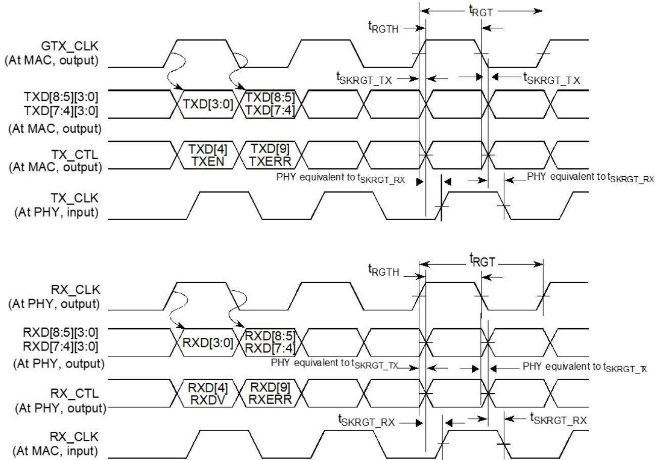
Figure 21. RGMII AC timing and multiplexing diagrams
