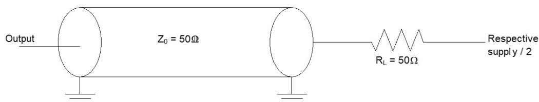
Figure 27. Integrated Flash Controller AC test load
