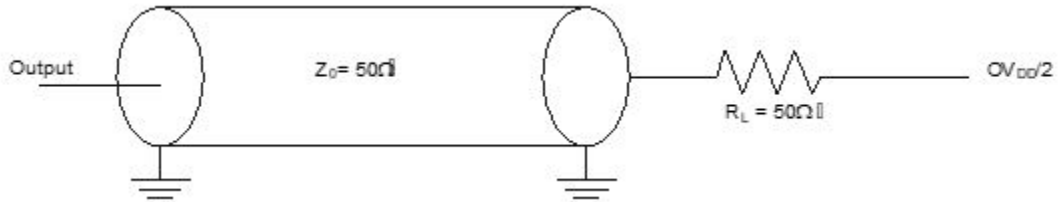
Figure 71. AC test load for the JTAG interface
