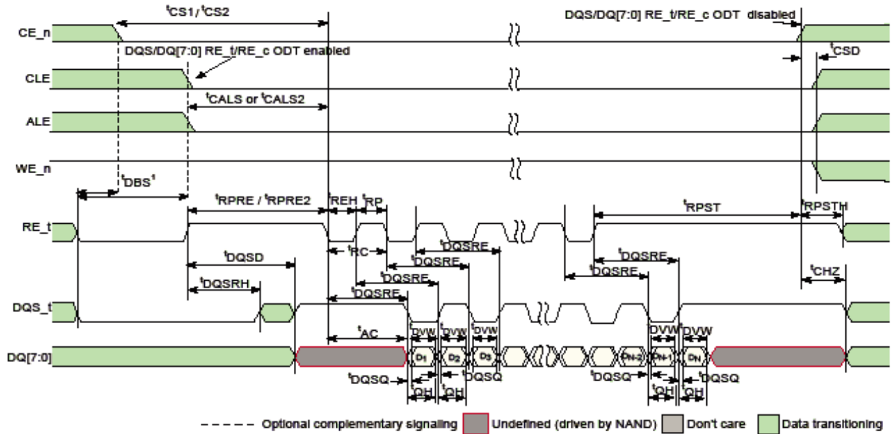
Figure 51. Read cycle
