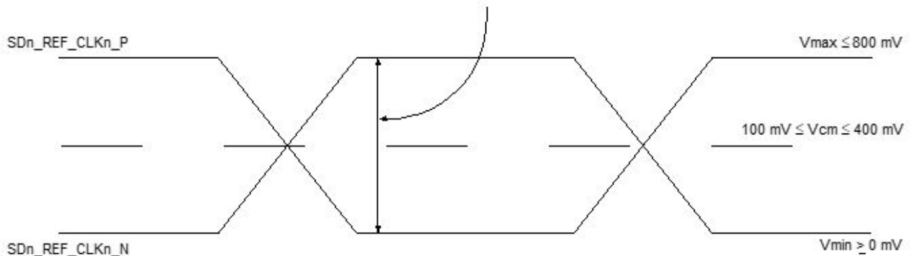
Figure 80. Differential reference clock input DC requirements (external DC-coupled)
