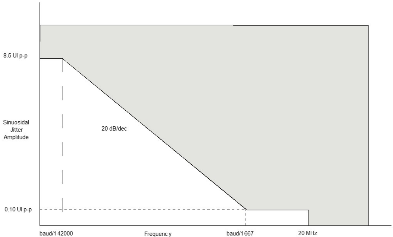
Figure 18. Single-frequency sinusoidal jitter limits
