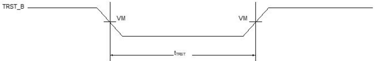
Figure 73. TRST_B timing diagram
