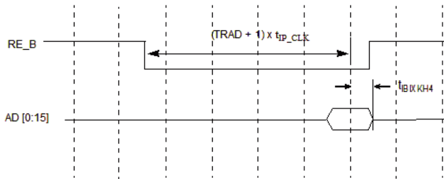
Figure 47. t_{BIXKH4} timings
