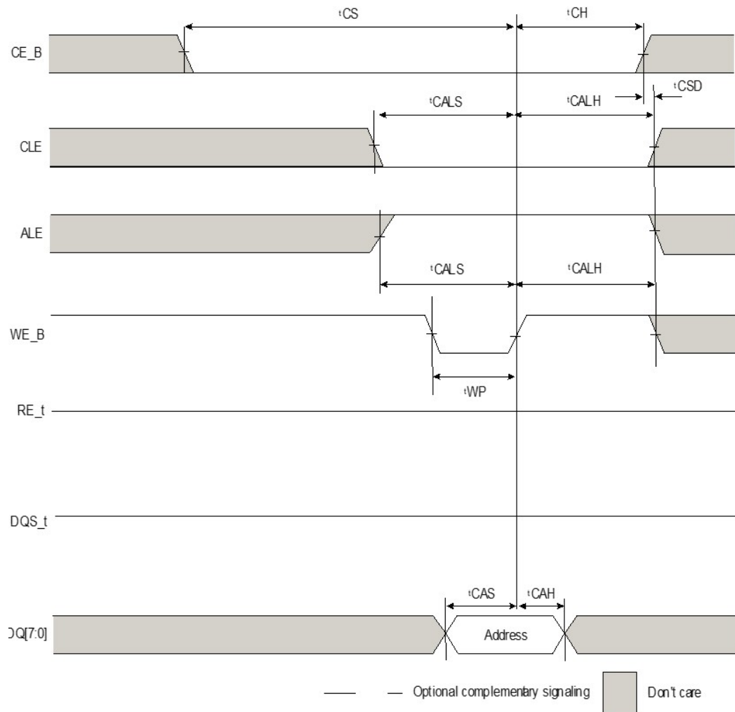
Figure 49. Address cycle
