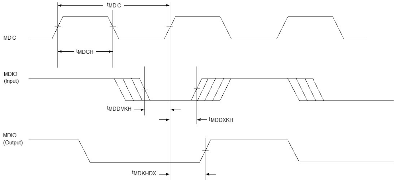
Figure 23. Ethernet management interface 2 timing diagram
