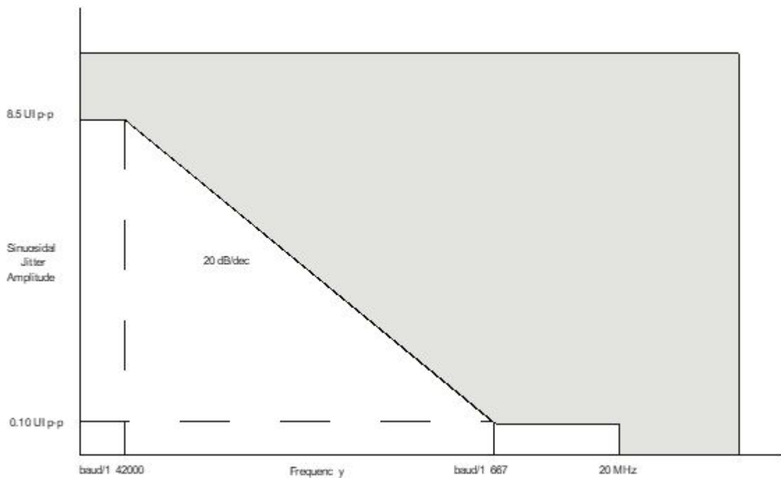
Figure 63. eSDHC high-speed mode input AC timing diagram
