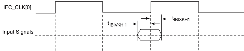
Figure 28. IFC-GPCM, IFC-GASIC input AC timing specifications
