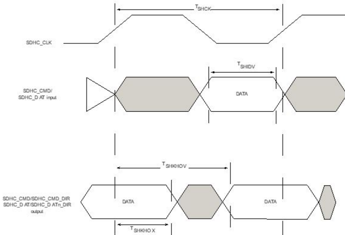
Figure 70. eSDHC SDR104/HS200 mode timing diagram
