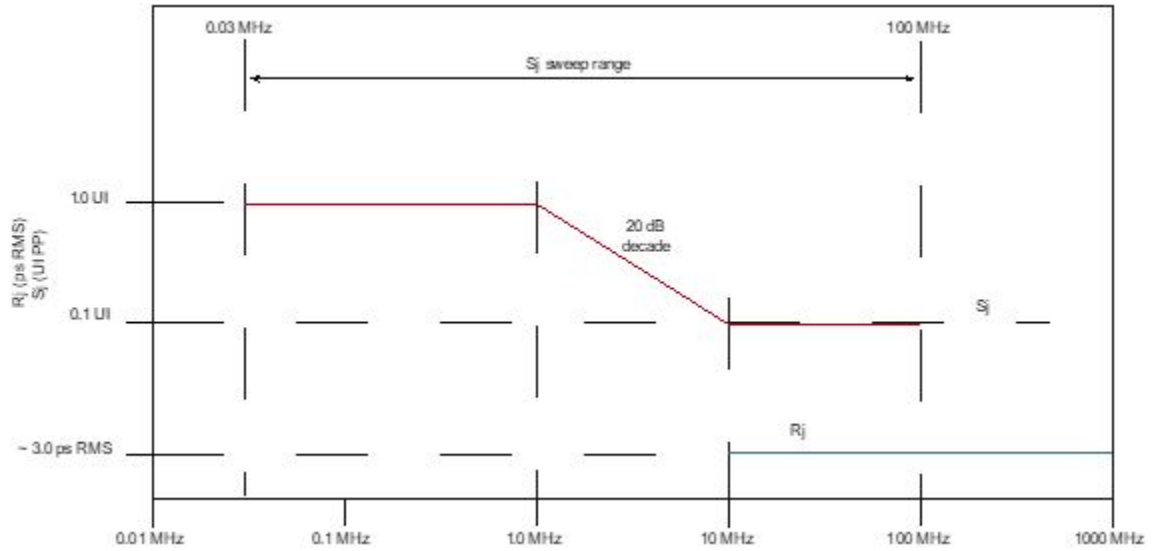
Figure 86. Swept sinusoidal jitter mask
