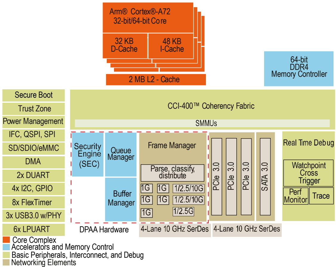
Figure 1. LS1046A block diagram
