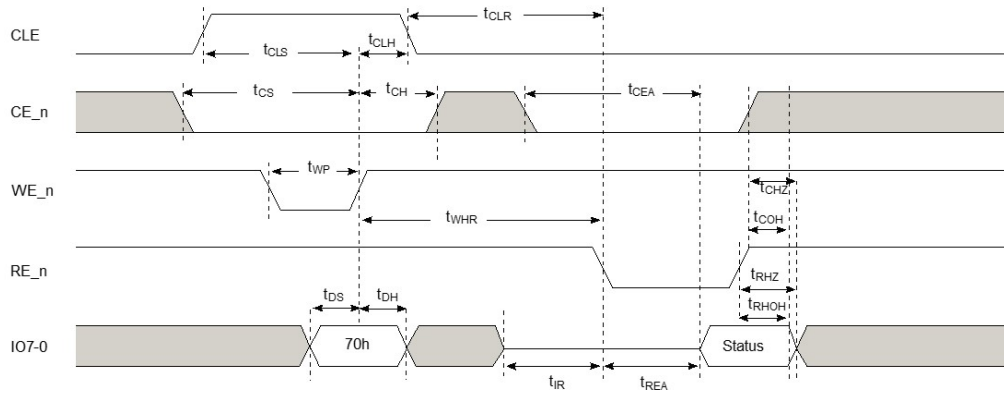
Figure 40. Read status timings
