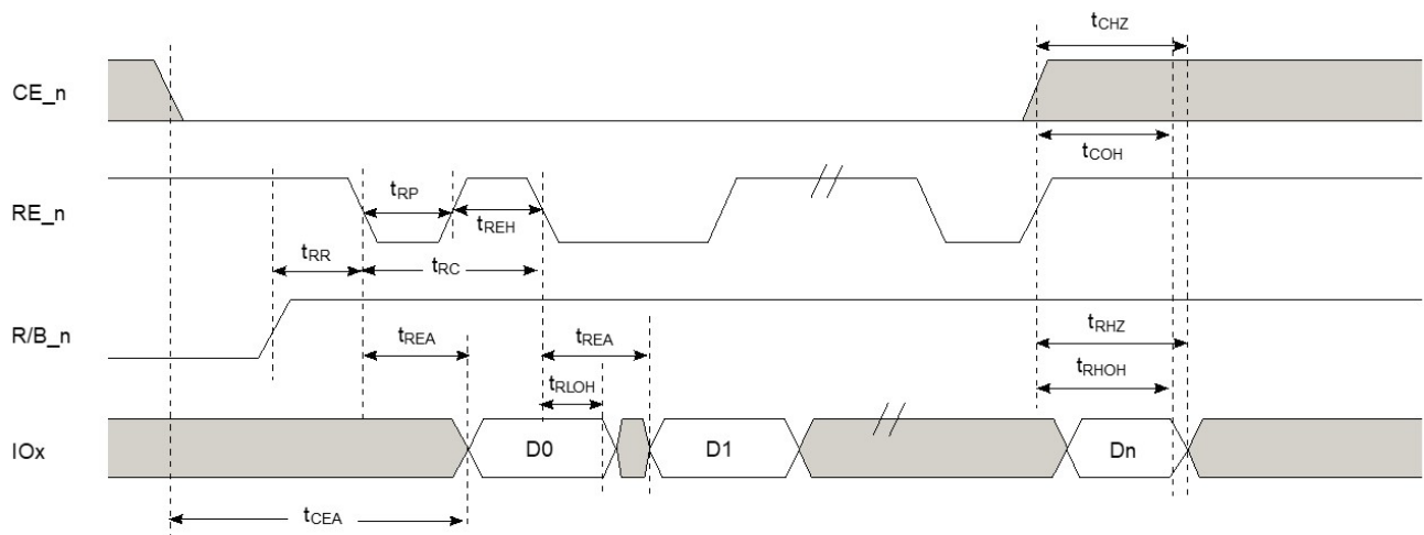
Figure 42. EDO mode data input cycle timings
