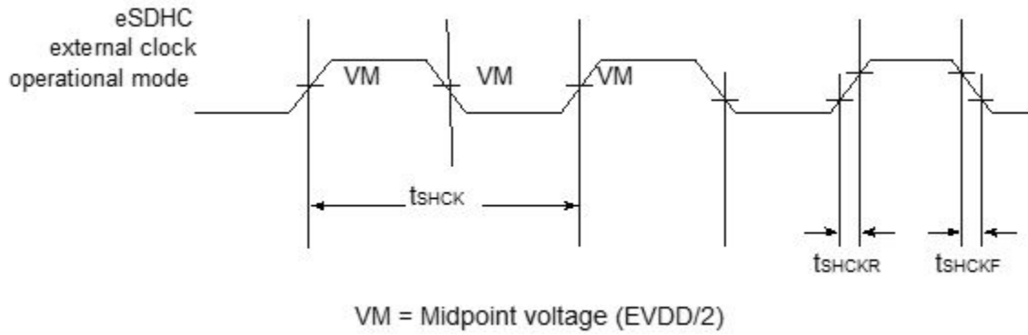
Figure 66. eSDHC SDR50 mode input AC timing diagram
