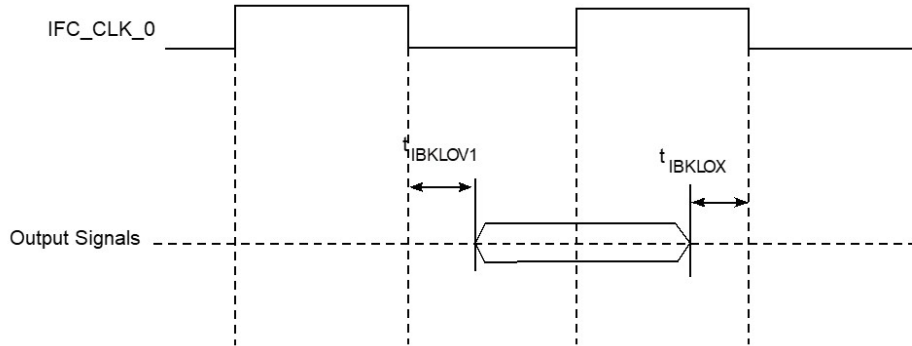
Figure 29. IFC-GPCM, IFC-GASIC signals
