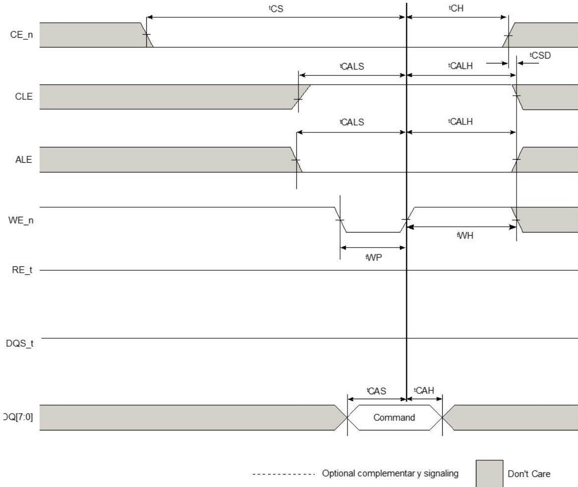
Figure 48. Command cycle
