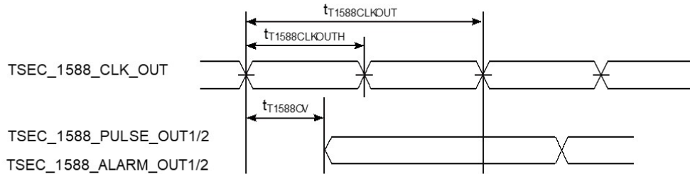
Figure 24. IEEE 1588 output AC timing
