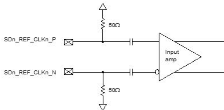
Figure 79. Receiver of SerDes reference clocks
