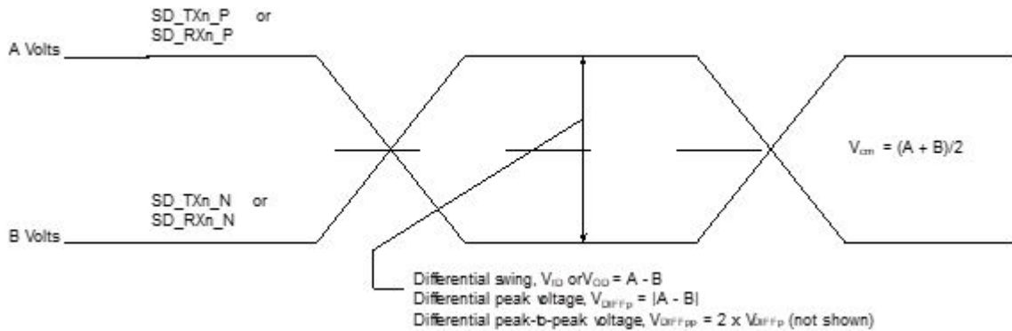
Figure 78. Differential voltage definitions for transmitter or receiver
