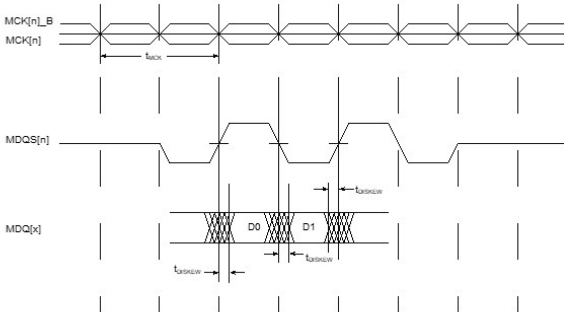
Figure 12. DDR4 SDRAM interface input timing diagram
