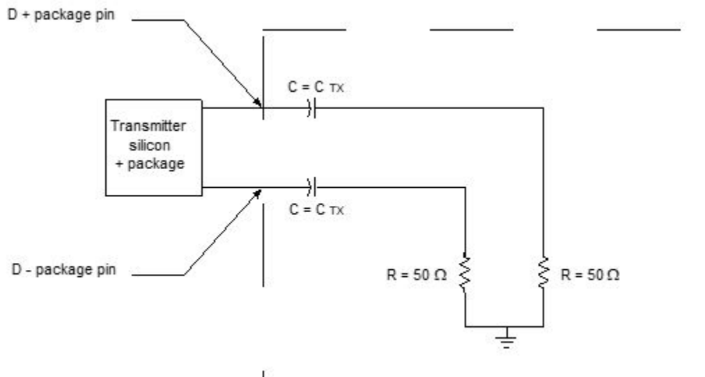
Figure 87. Test and measurement load
