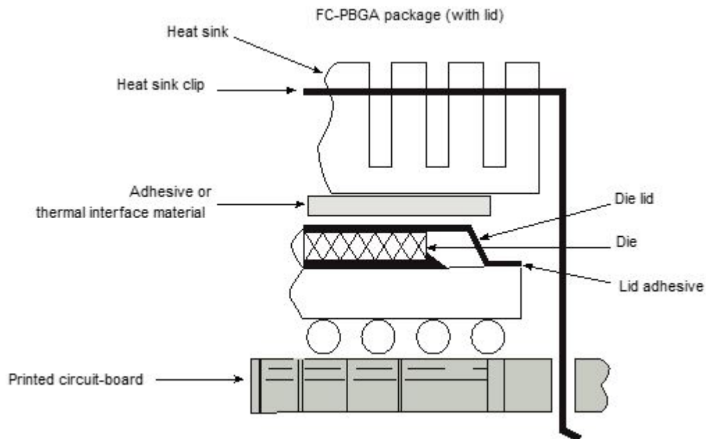
Figure 91. Package exploded, cross-sectional view-FC-PBGA
