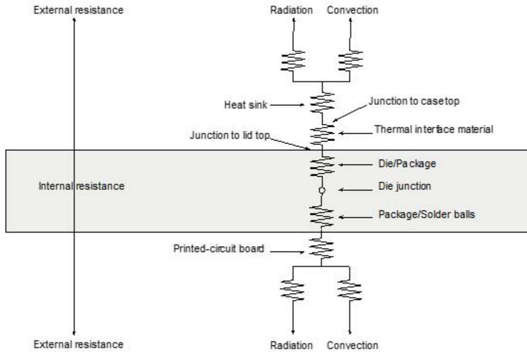
Figure 92. Package with heat sink mounted to a printed-circuit board
