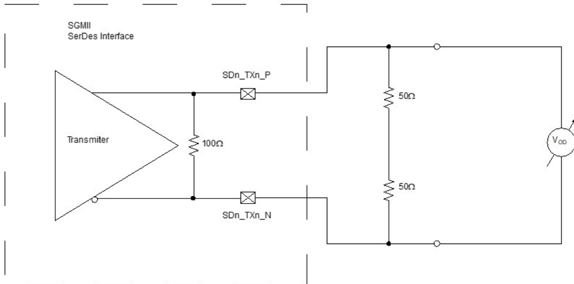
Figure 16. SGMII transmitter DC measurement circuit
