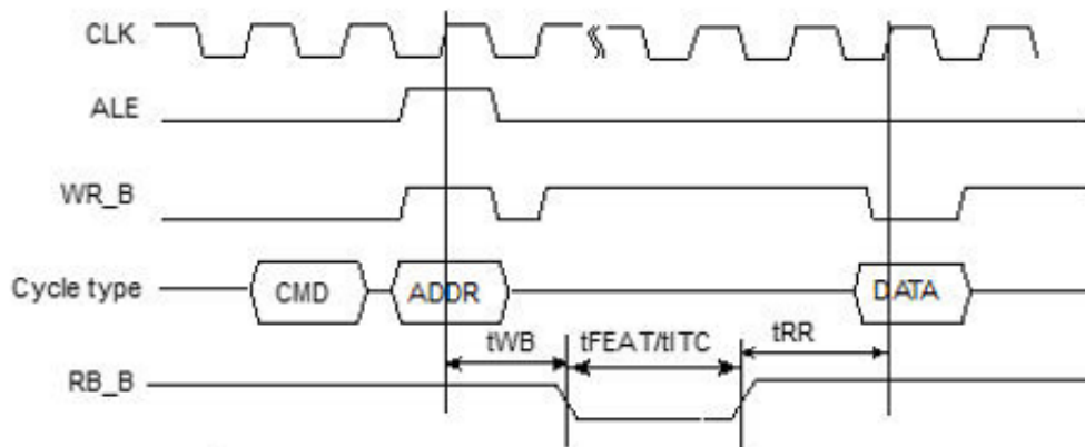
Figure 39. t_{WB} , t_{FEAT} , t_{ITC} , and t_{RR} timings
