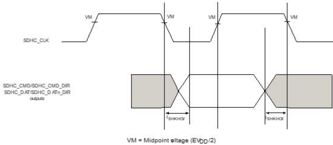
Figure 64. eSDHC high-speed mode output AC timing diagram
