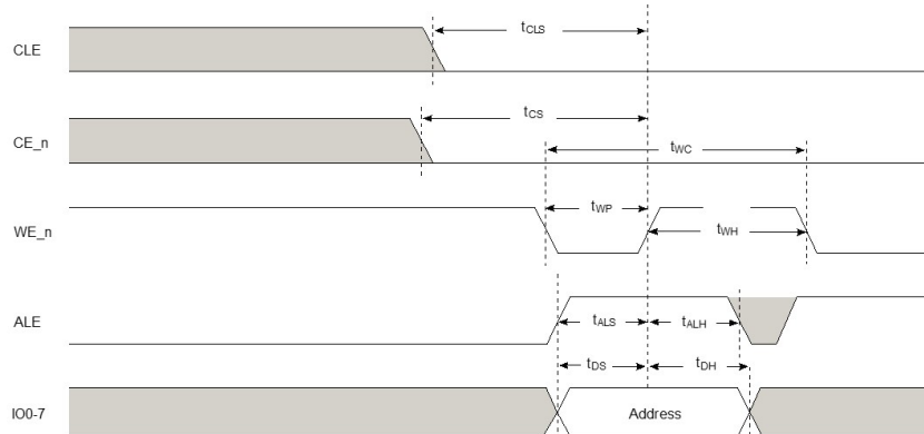
Figure 44. Address latch timings
