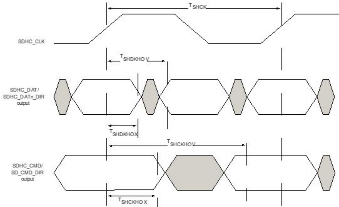
Figure 69. eSDHC DDR50/DDR mode output AC timing diagram
