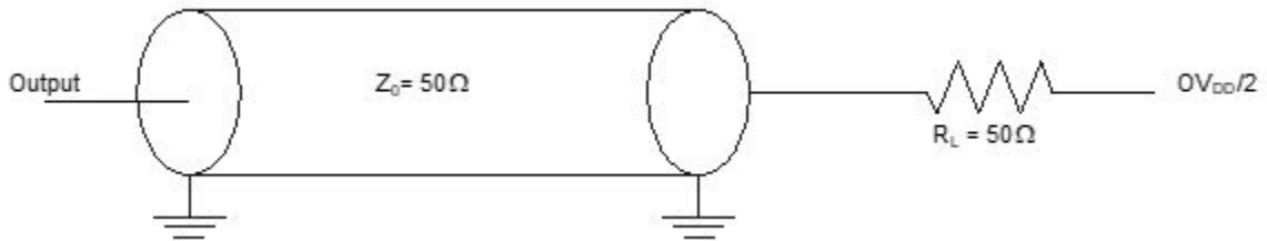
Figure 75. I 2 C AC test load
