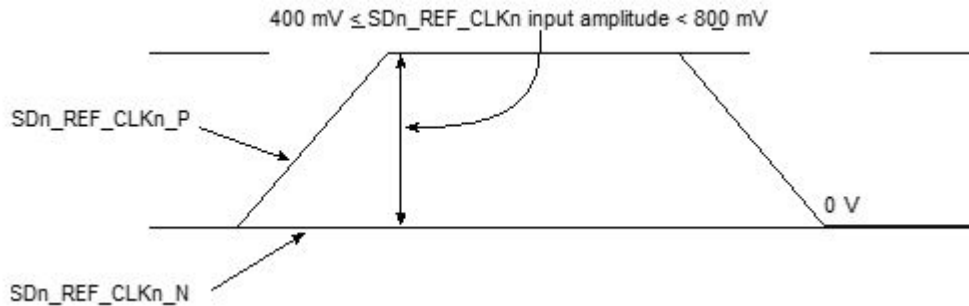
Figure 82. Single-ended reference clock input DC requirements
