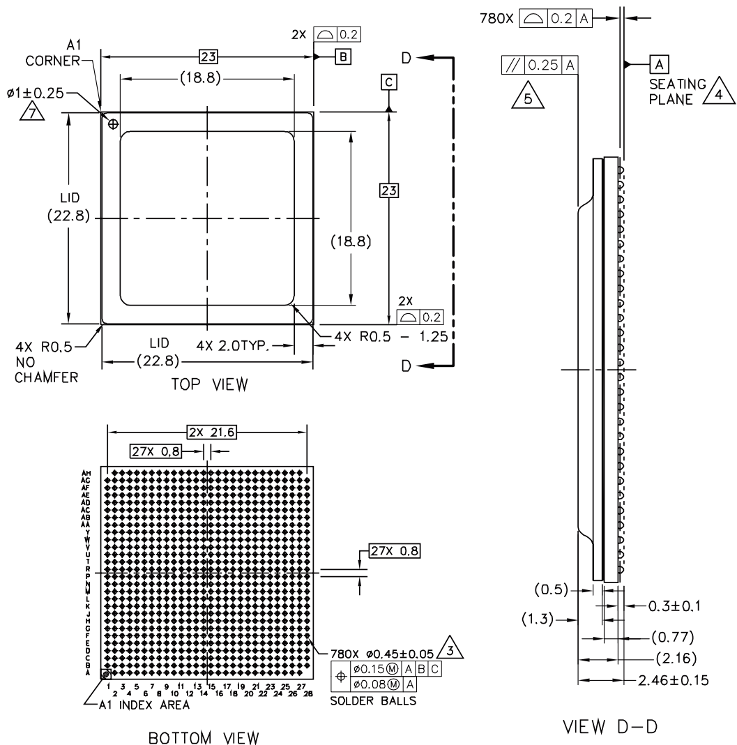
Figure 93. Mechanical dimensions of the FC-PBGA
