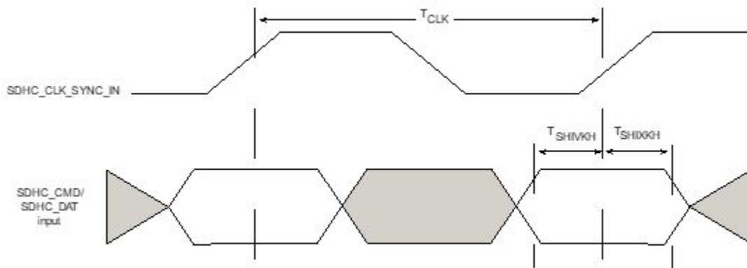
Figure 66. eSDHC SDR50 mode input AC timing diagram
