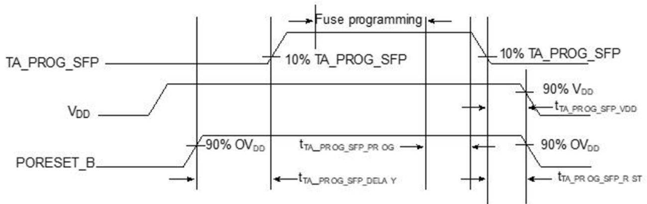
Figure 9. TA_PROG_SFP timing diagram
