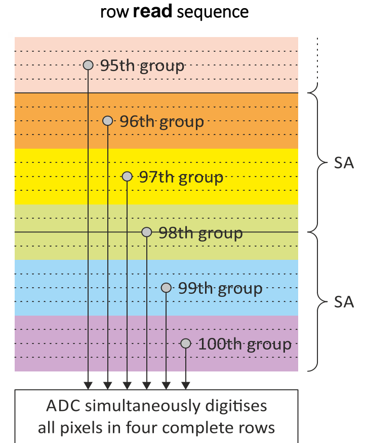
Figure illustrates last 24 rows and adjacent ADC block. Figure is for lower half of LVSM. Upper half is a mirror image.
